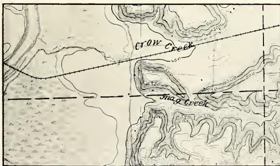
B. Map showing stream piracy east of Chillicothe. (Portion of Metamora topographic map, U. S. Geol. Surv.)
